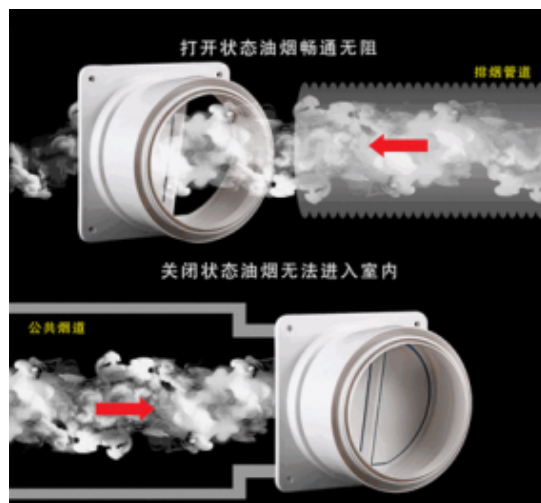
止回阀
